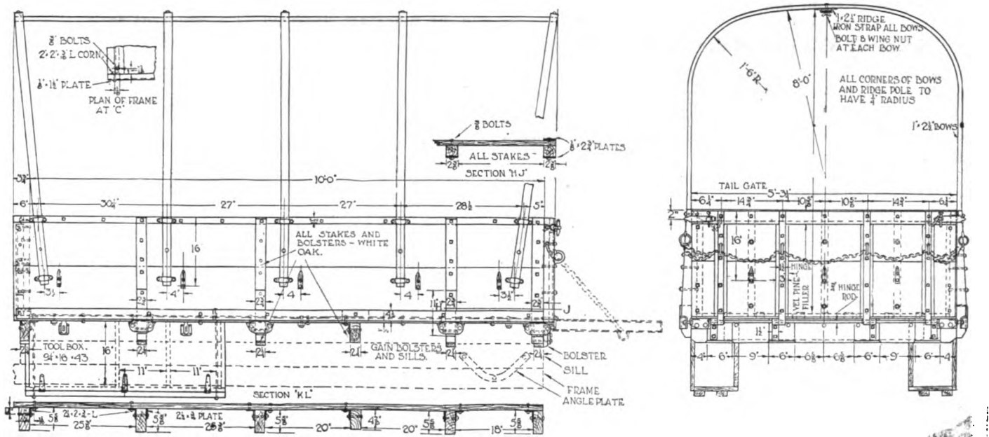
CLASS A MILITARY TRUCK
